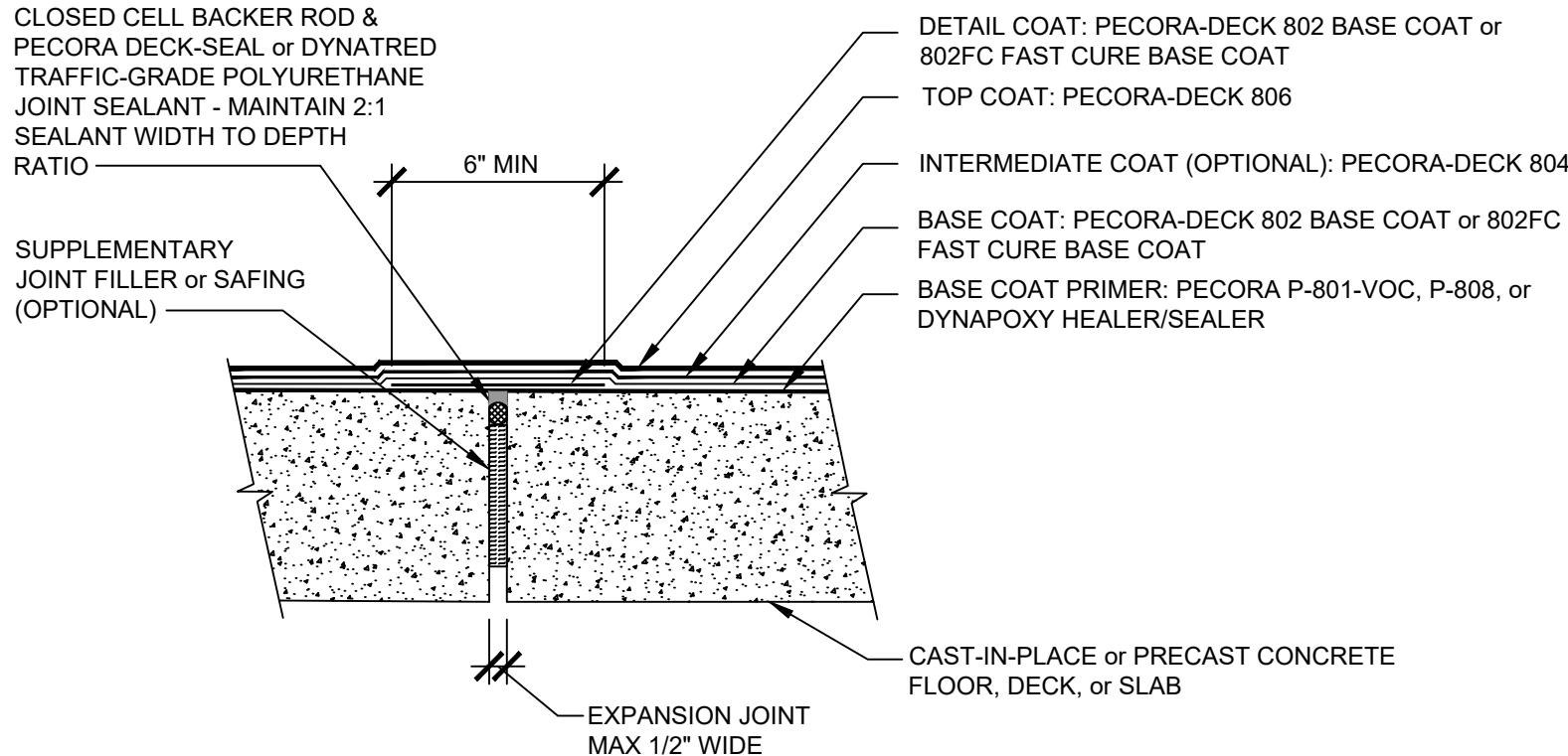
104: EXPANSION JOINTS UP TO 1/2" WIDTH
