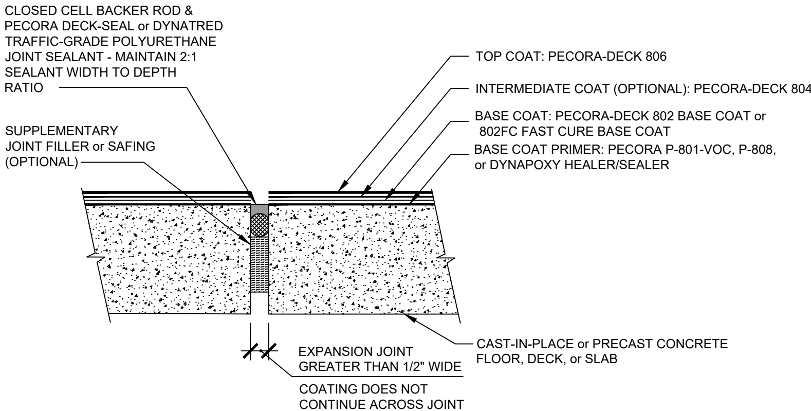
105: EXPANSION JOINTS > 1/2" WIDTH
